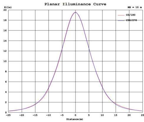
Illumination Curve
