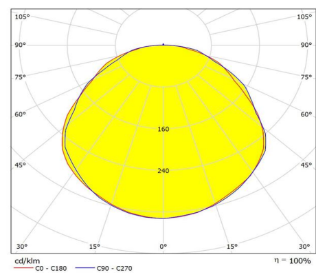
Luminance Distribution
