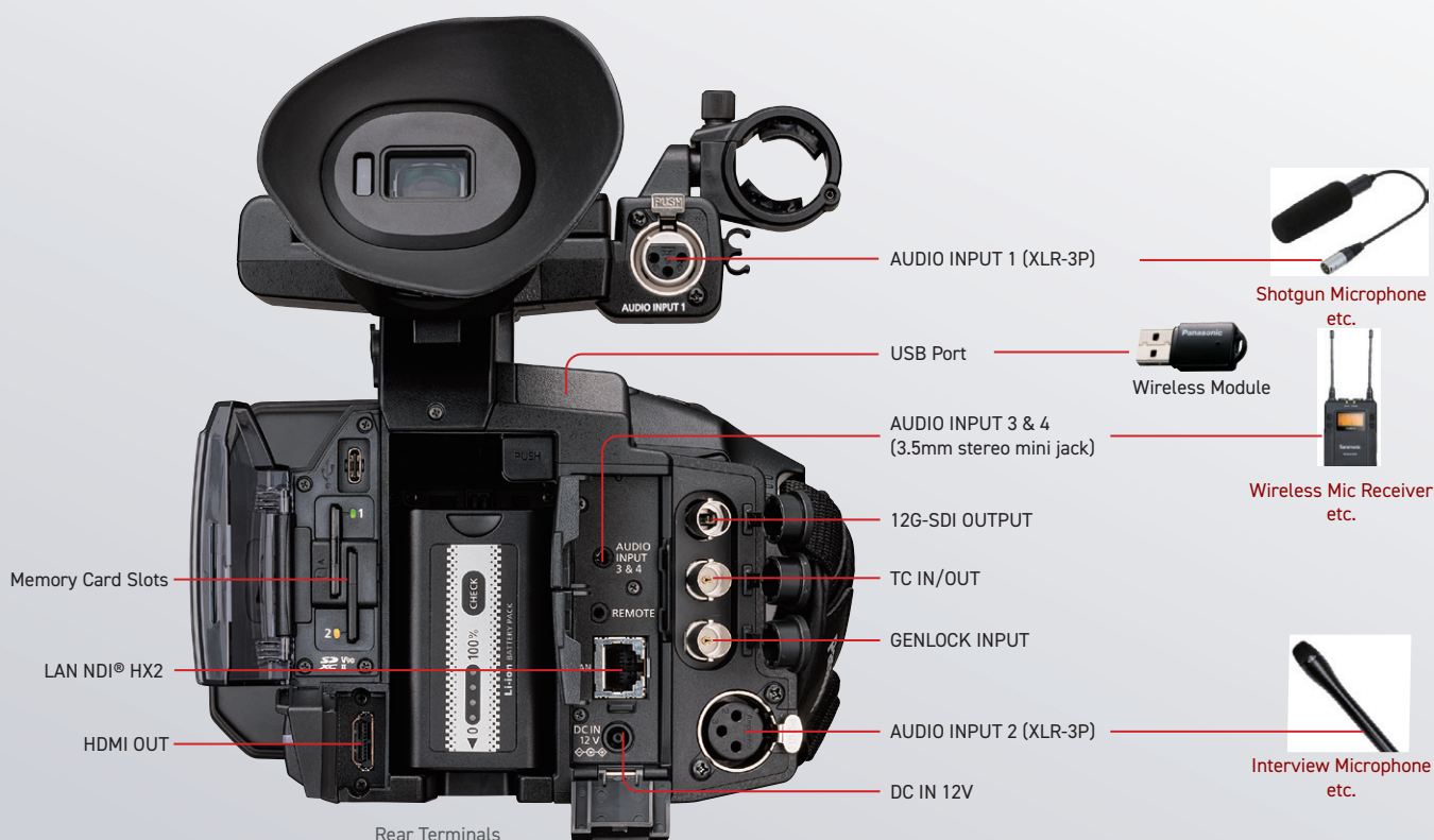
Rear Terminals
