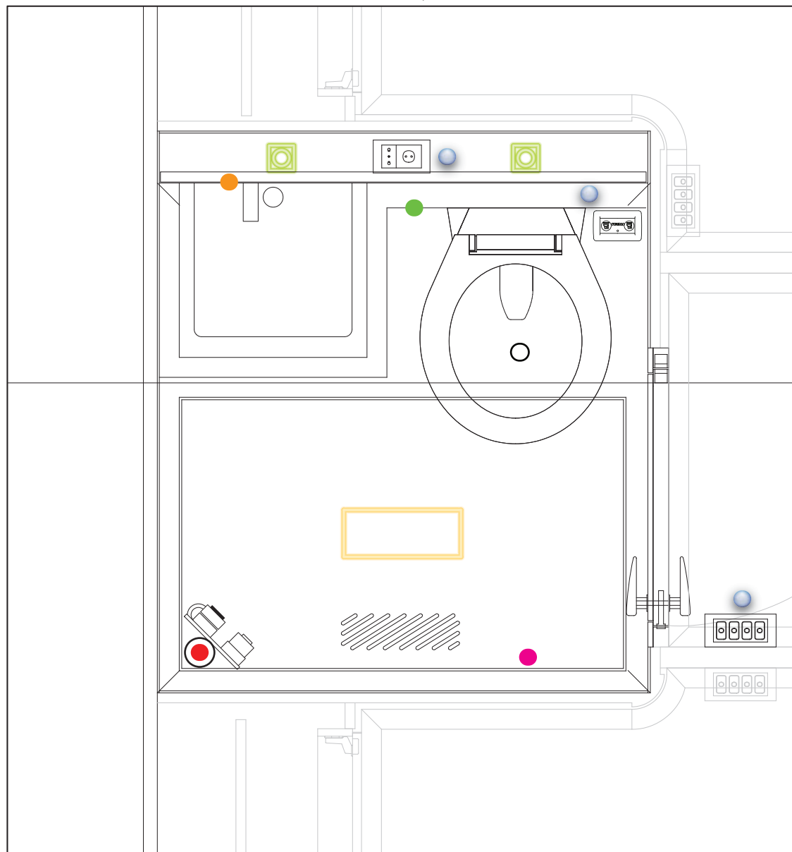
guest head layout
