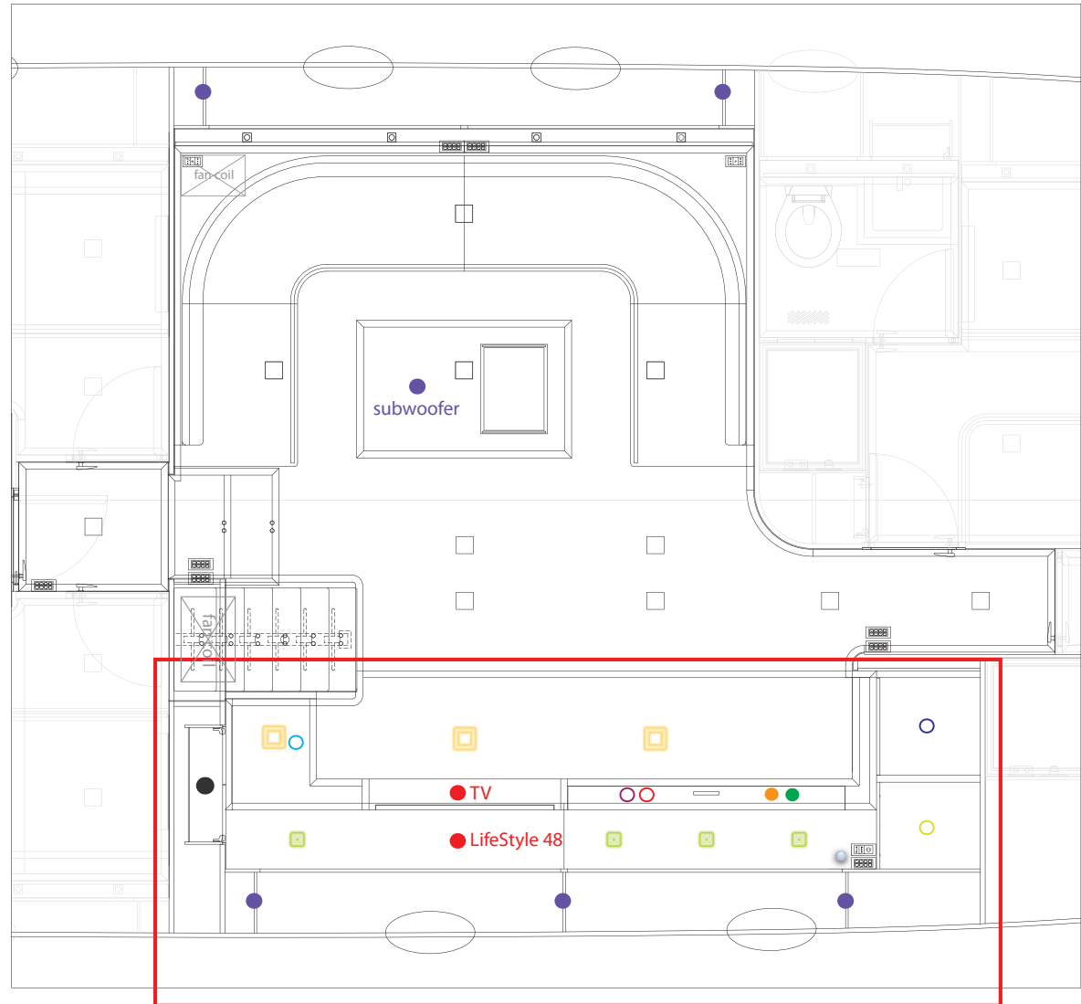
Galley layout
