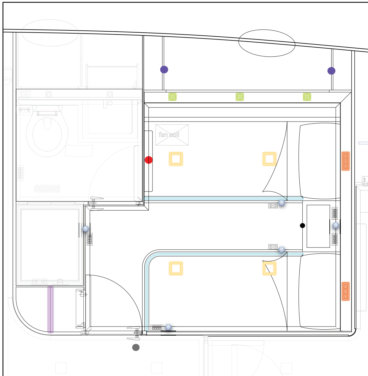
Vip state room layout
