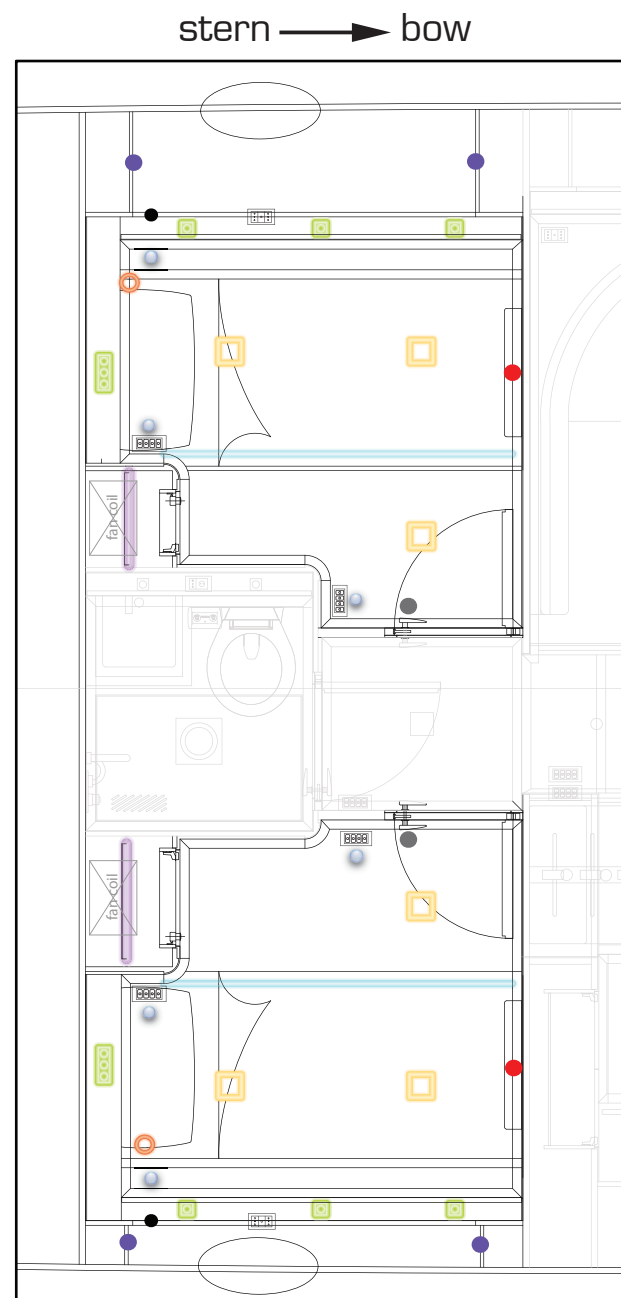
Guest state rooms layout
