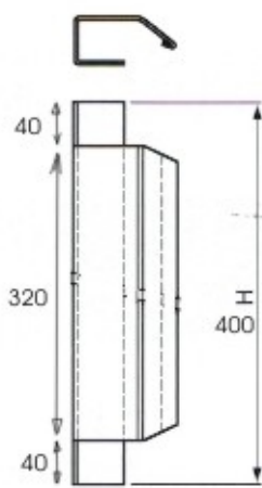
art. 44144 TESTATA H 400 ANT/POST
