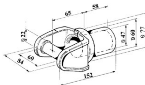
art. 25310 FORCELLA D. 60 gr. 1.650
