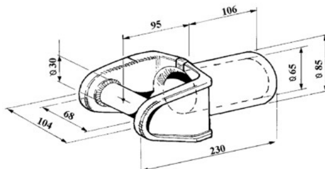
art. 25320 FORCELLA D. 85 gr. 4.900
