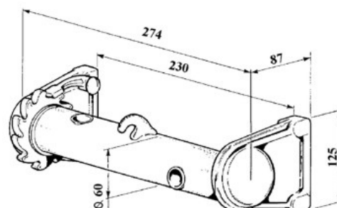
art. 30142 VERRICELLO D. 60 SUPP. STAMPATI C/TUBINO gr. 4.240
