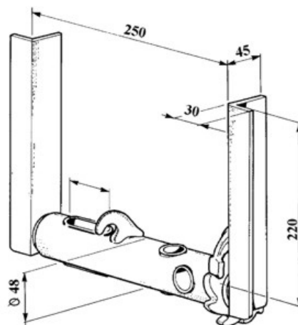
art. 30204 VERRICELLO D. 48 STAFFE 220 C/TENDINASTRO gr. 2.340
