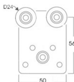
art. 46280 CARRELLO ZINC.4 CUSC. gr. 125 PORTATA Kg. 50
