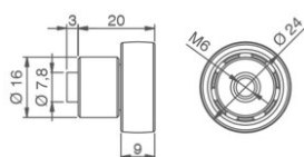
art. 46814 CUSCINETTO SESAM gr. 100
