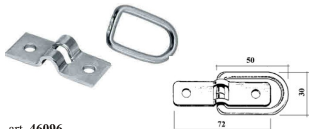
art. 46096 ANELLO TIR ORIENTABILE gr. 35
