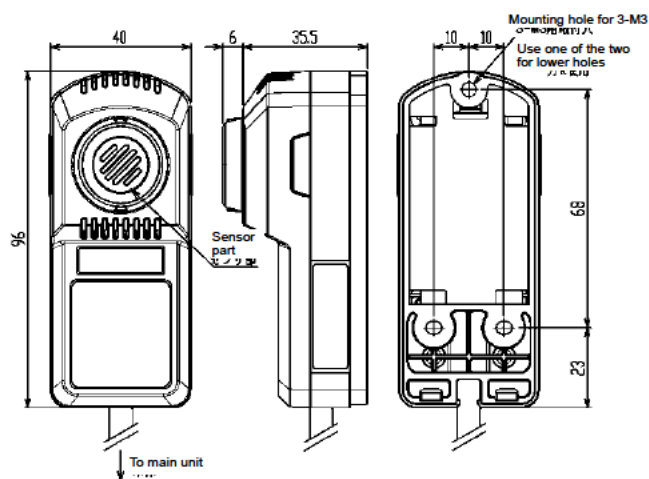
Remote sensor
