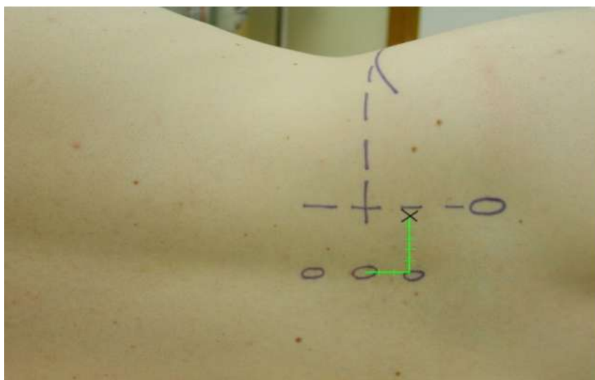
Figure 3. Chayen’s approach.
