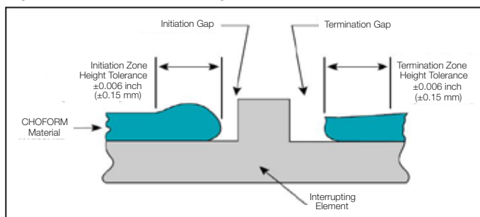
Figure 7-3 Side View Gasket height tolerances
