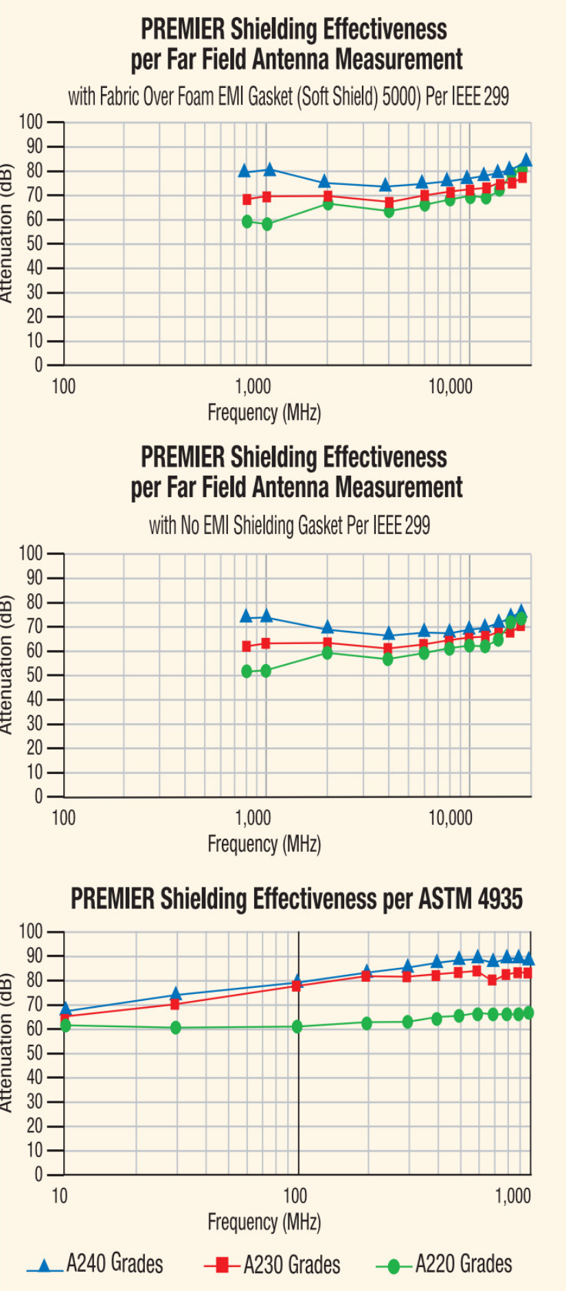
Figures 6-8: PREMIER shielding effectiveness performance
