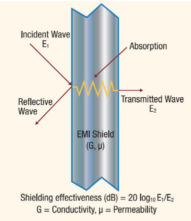
Figure 4: Shielding Effectiveness
