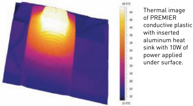
Figure 9: Effective thermal management with 10W source
