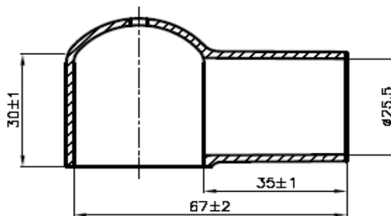
Section A-A(1:1)
