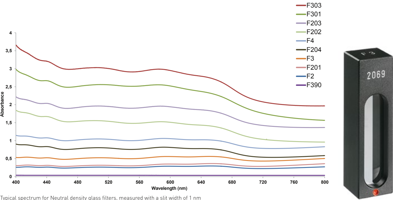
Typical spectrum for Neutral density glass filters, measured with a slit width of 1 nm
