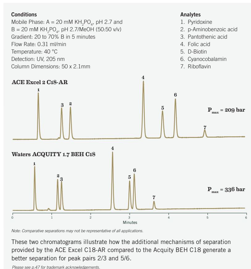
FIGURE 22: Leveraging ACE Excel C18-AR Selectivity
