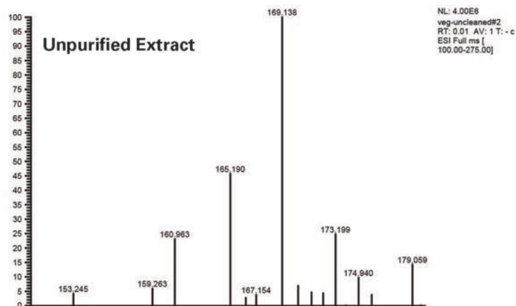
Glyphosate Ionization Region 150-180 m/z
