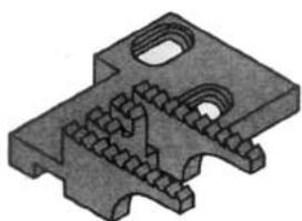
15-7310-0 Griffa posteriore
