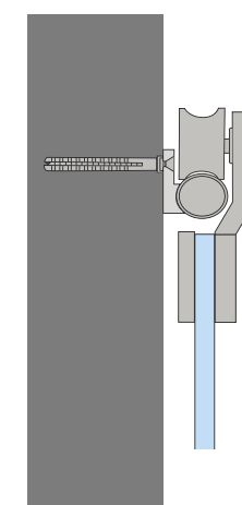
Binario TRIO TRIO track
