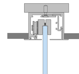
Binario FILOMURO WALL FILOMURO WALL track
