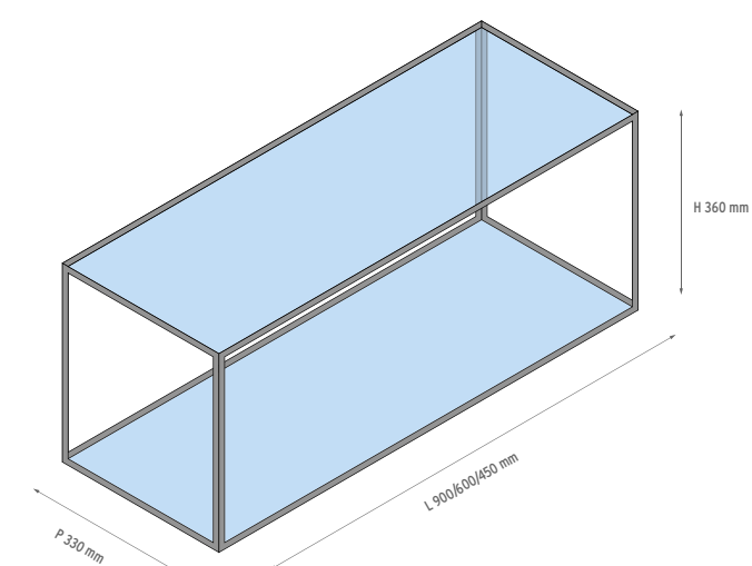
Box con mensole in vetro Box with glass shelves
