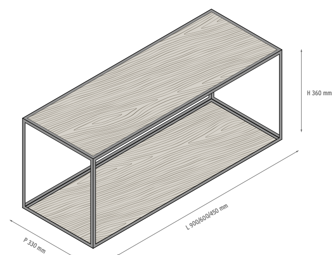
Box con mensole in legno Box with wood shelves
