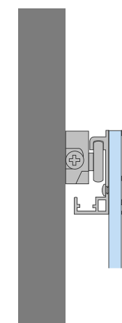
Binario ROLLER ROLLER track
