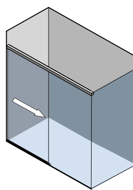
KIT 2 - MURO / VETRO KIT 2 - WALL / GLASS
