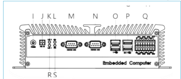
Rear Panel External I/O Mechanical Layout/Drawing
