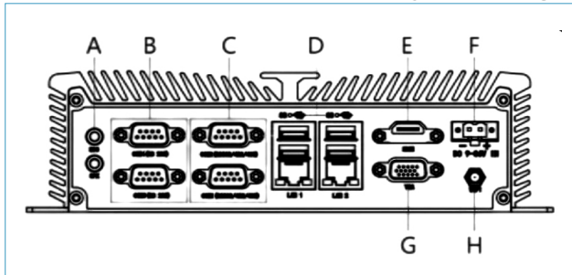
Front Panel External I/O Mechanical Layout/Drawing
