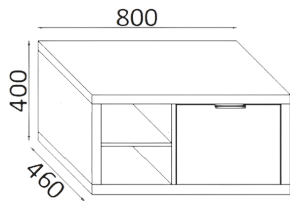
Base 1 cassetto dx + vano a giorno Base 1 drawer dx + open compartment
