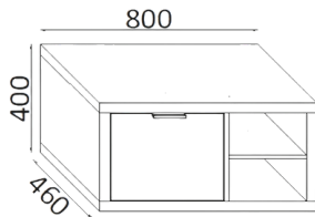
Base 1 cassetto sx + vano a giorno Base 1 drawer sx + open compartment
