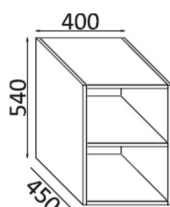
Base a giorno Lateral cabinet with shelves
